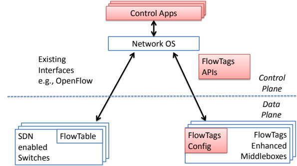
Figure 4: The FlowTags architecture: We highlight the extensions we introduce as part of FlowTags. We avoid explicit changes to switches or the need for direct interfaces between switches and middleboxes.
